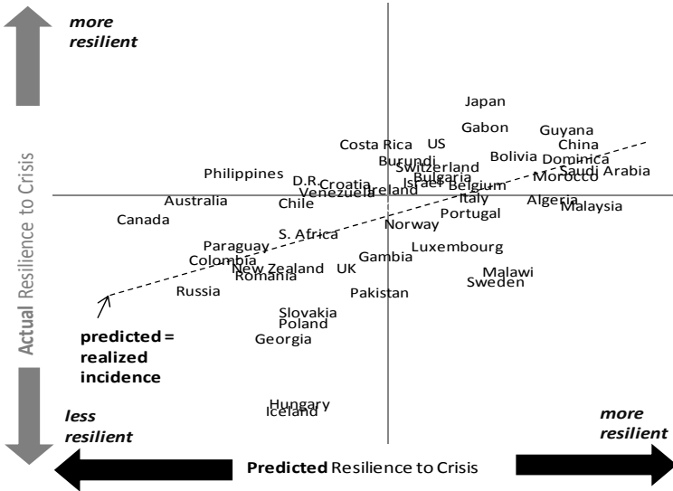
Figure 4: Success at predicting the impact of the 2008-09 crisis
